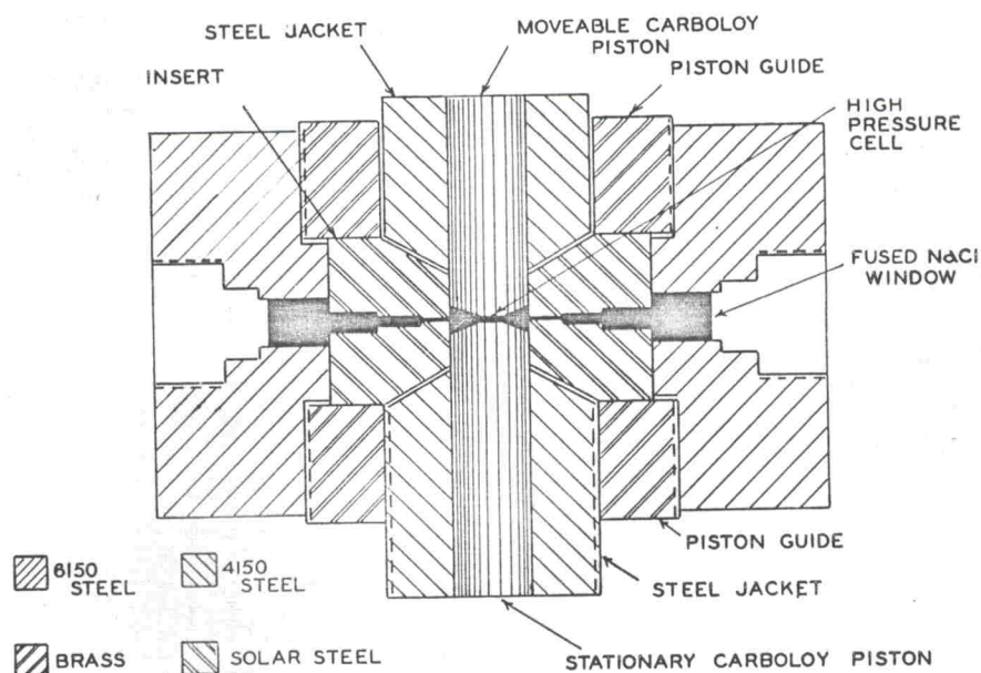
Fig. 2 Diagram of 0-250,000 atm pressure cell.
